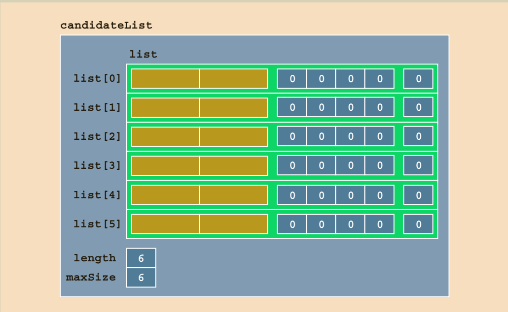
FIGURE 18-41 candidateList
