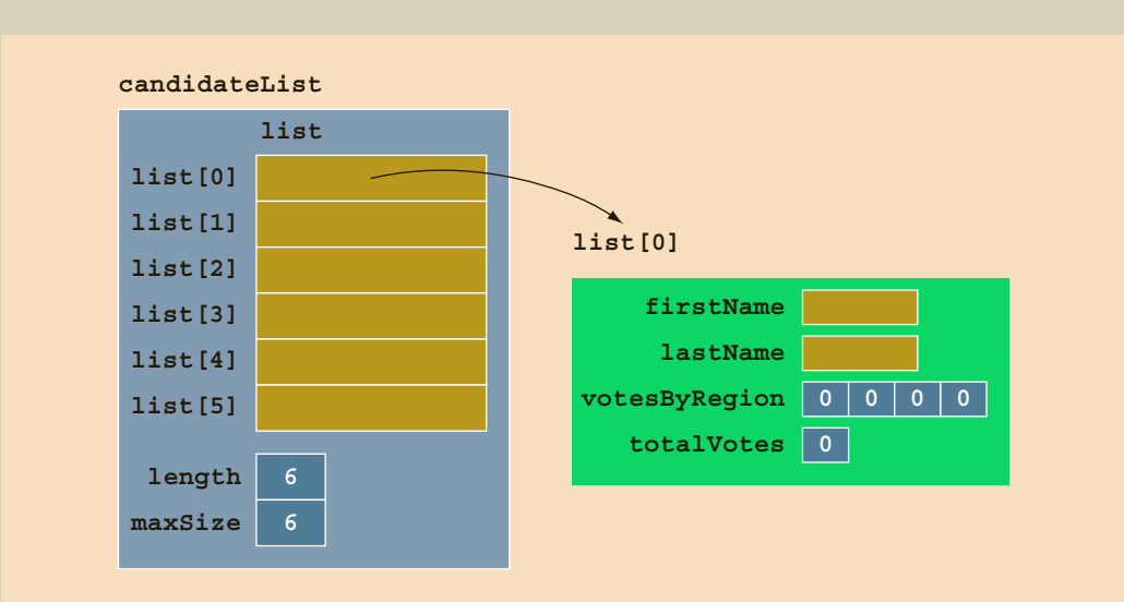
FIGURE 18-40 candidateList
