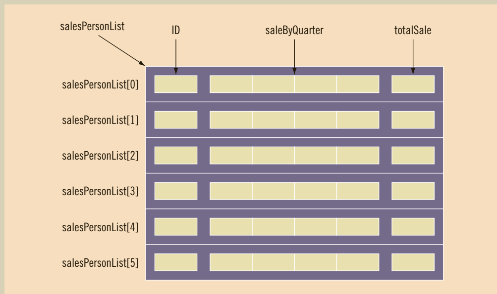
FIGURE 9-9 Array salesPersonList
